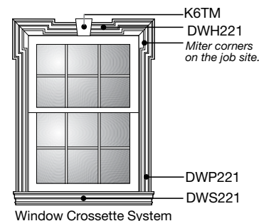
Window Crossette System
