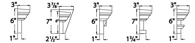
Standard w/ Keystone K6M^ w/ Dentil Trim w/ Bottom Trim w/ Trim Strip
